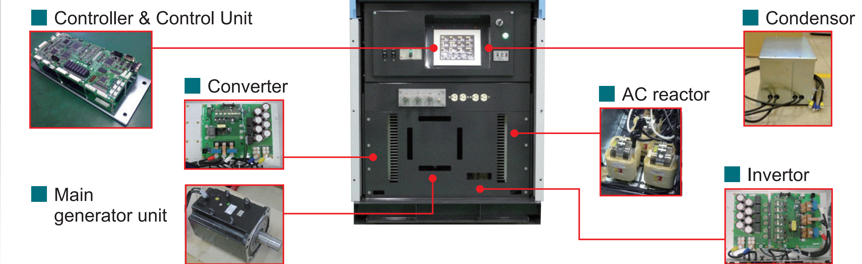
VS Generator (VSG28A) Awarded ten best new products of the year prize by Nikkan Kogyo Shinbun along with Hokuetsu Industries Co., Ltd. and Toshiba Industrial Products and Systems Corporation
